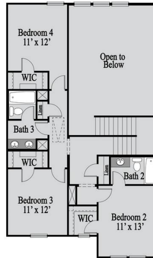
SECOND FLOOR
